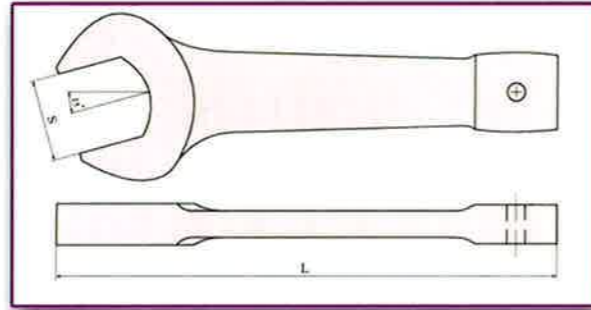
Striking open end wrench Maulschlüssel, DIN 133 Llave de Boca de Golpe
