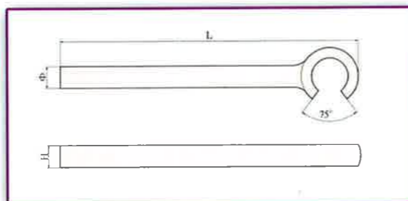
Wrench,C Lenkradschlüssel Clave a volante
