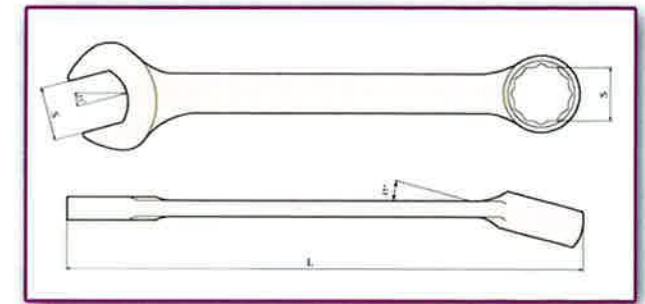
Combination wrench Ringmaulschlüssel DIN 3113 Llave Combinada
