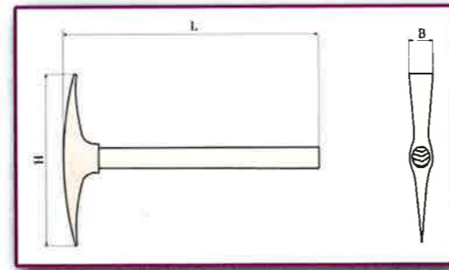
Railroad pick Kreuzhacke, DIN 20109 Pico de Ferrocarril
