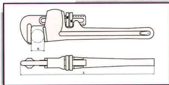
Adjustable pipe wrench Verstellbarer Rohrschlüssel Llave Adjustable para Tubos
